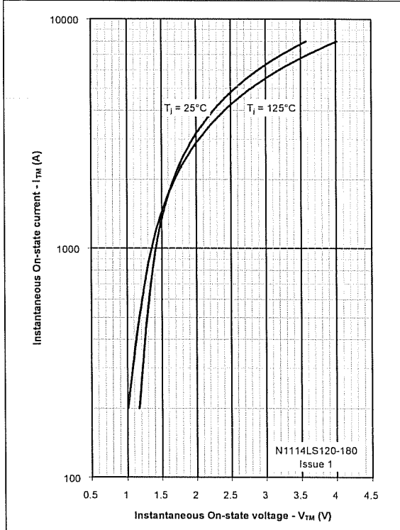
Figure 9 - On-state characteristics of Limit device
